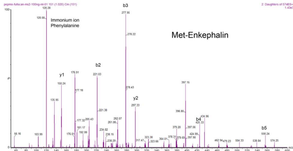
Figure 3B : MS/MS fragmentation spectrum of Met-enkephalin,
