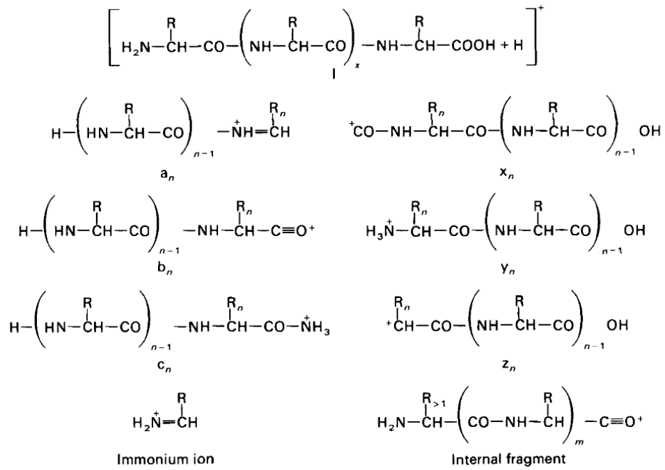
Schéma A1. Fragments produced from protonated linear peptides (I) by cleavage of a peptide bond independent of R.
